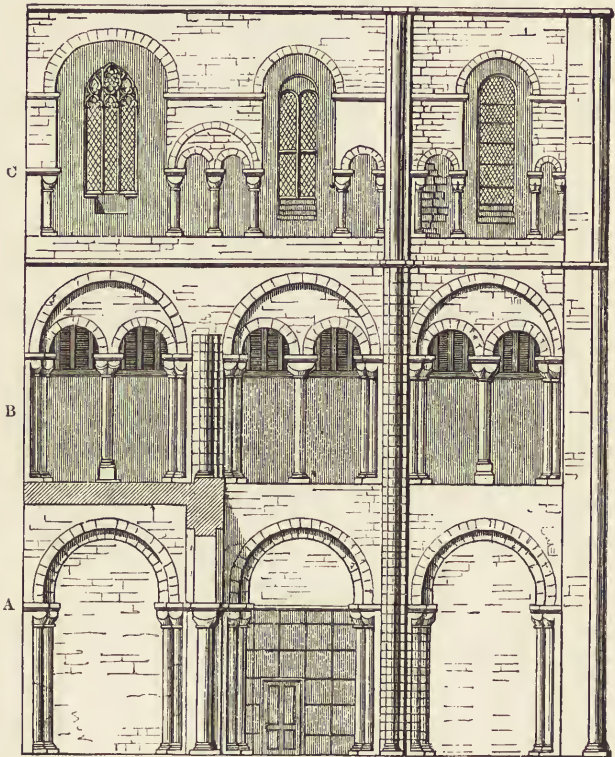
28. Transept, Winchester Cathedral, A.D. 1079—1093.
